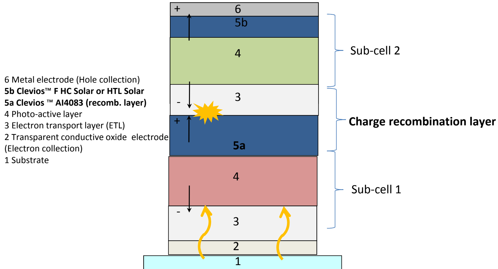
Figure 3: OPV Inverted Tandem Cell Architecture
